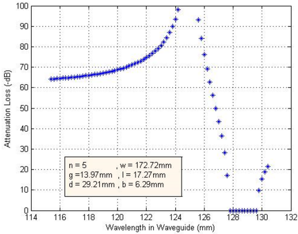
Figure 7. Attenuation loss of the doubly corrugated filter with the parameters from Metaxas et al. (1993).
