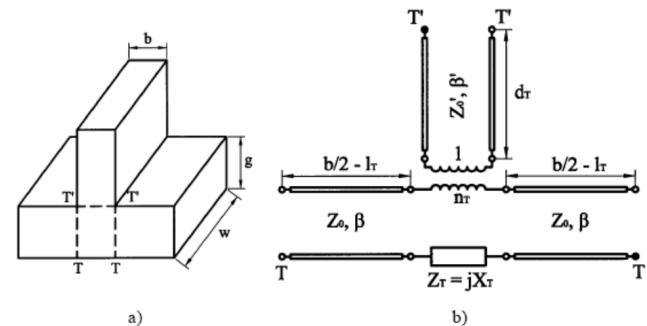
Figure 3. (a) General view and (b) equivalent circuit of E-plane T-junction.
