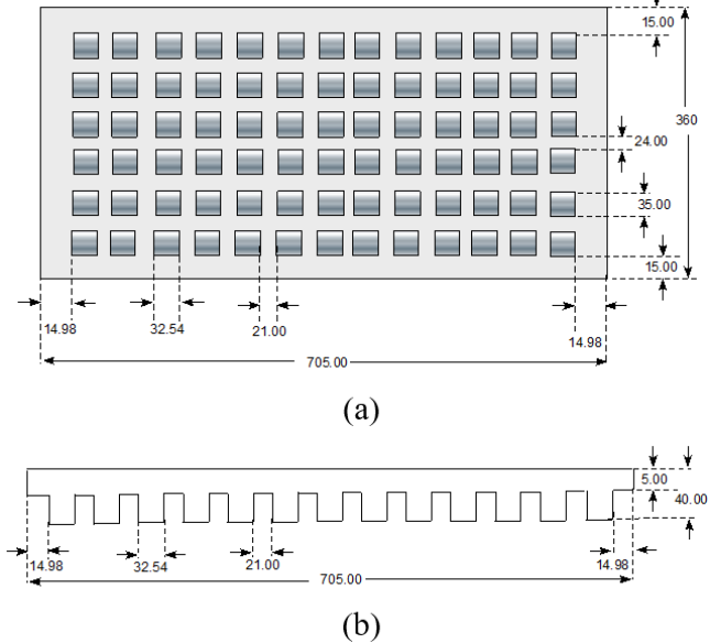
Figure 8. General schematics of the R.C.M.E. doubly corrugated filter, (a) bottom view (b) side view.
