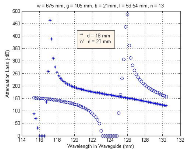
Figure 6. Attenuation loss of the doubly corrugated filter when g and d parameters are varied.
